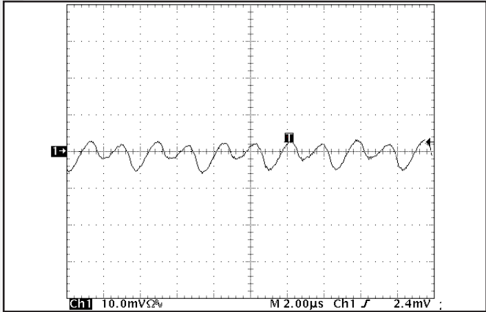
Figure 10: Input Terminal Current Ripple, i_c , at full rated output current and nominal input voltage. Bandwidth: 2MHz. See Figure 17. Ch 1: i_c (200mA/div), Time (2µs/div).
